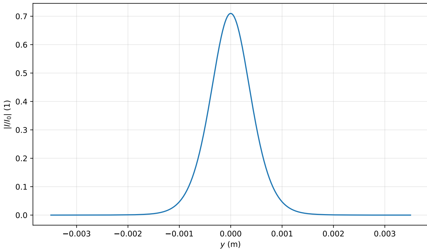
Intensity profile I(x=0, y, z=2.866)/I_0 , P_{in}=0.6P_{cr} , artificial time
